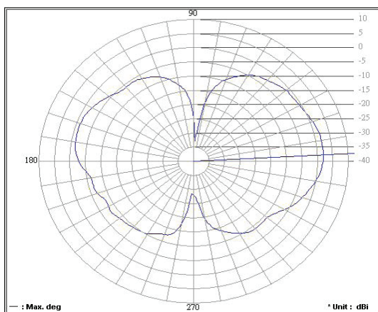
Antenna pattern 2.4 GHz - horizontal
