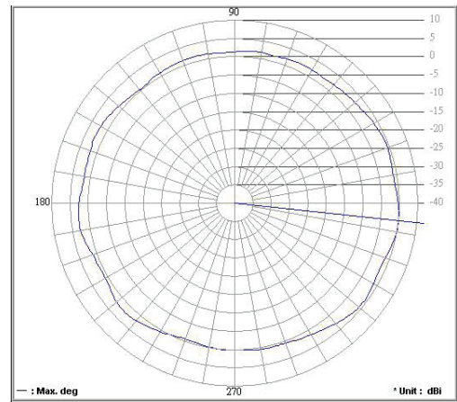
Antenna pattern 5 GHz - vertical
