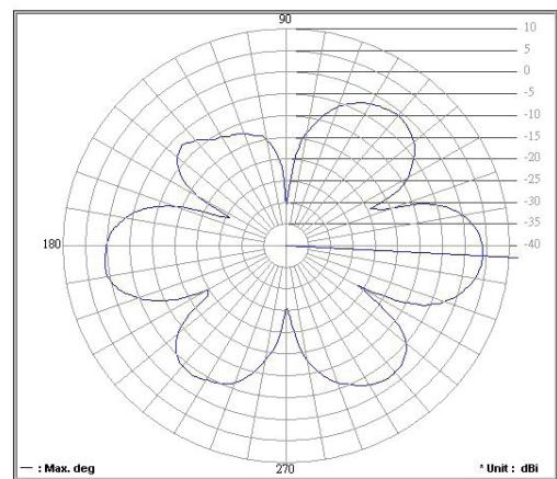
Antenna pattern 5 GHz - Horizontal
