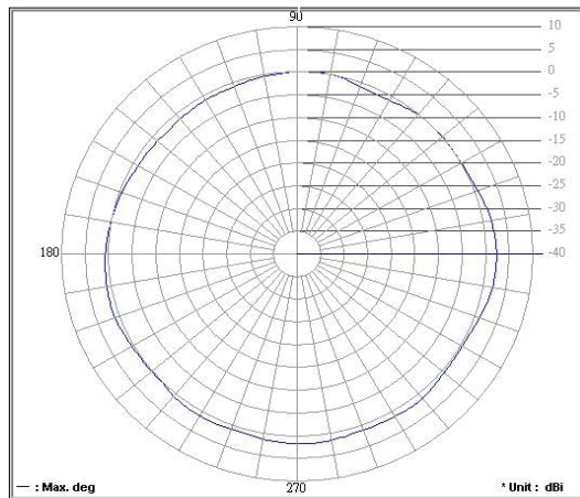
Antenna pattern 2.4 GHz - vertical
