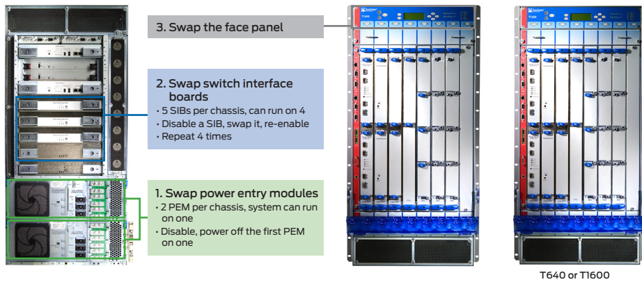
Figure 3: The in-service hardware upgrade of T640 to T1600
