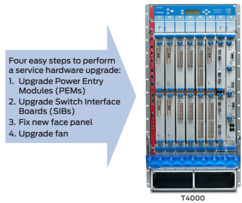
Figure 4: The in-service hardware upgrade of T640/T1600 to a T4000 system.
