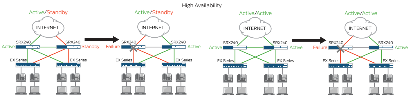
Figure 2: High availability
